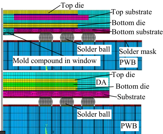
Figure 15: Quarter model for D2-wCSP
