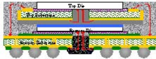
Figure 5: 2DD2-wCSP package structure with both dice facing package bottom direction
